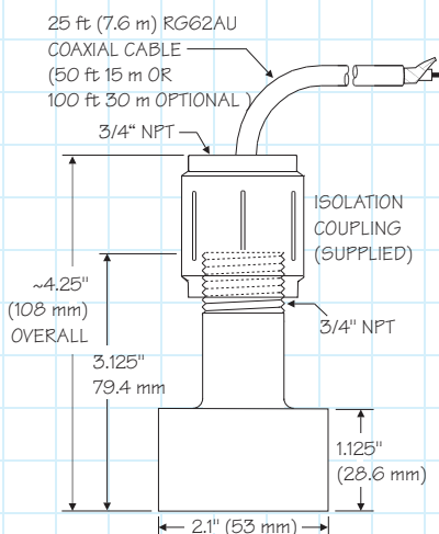
PZ15 SENSOR
